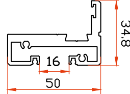
SLP-027 Pattam [ 50x16 ]
