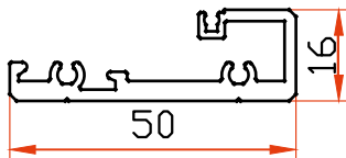
SLP-S-FV Cover
