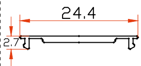
SLP-S-VC Vertical Cover
