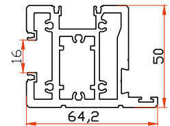
SLP-S-3WGE 3 Way Glass L Enclosure
