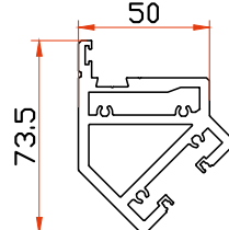
SLP-S-135°M 135° Shower
