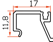
SLP-S-FVC Cover
