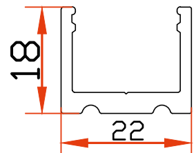
SLP-S-UC U Cover (18mm)
