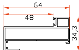
SLP-QF-45 Pattam
