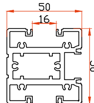
SLP-S-90° Vertical Profile 90°
